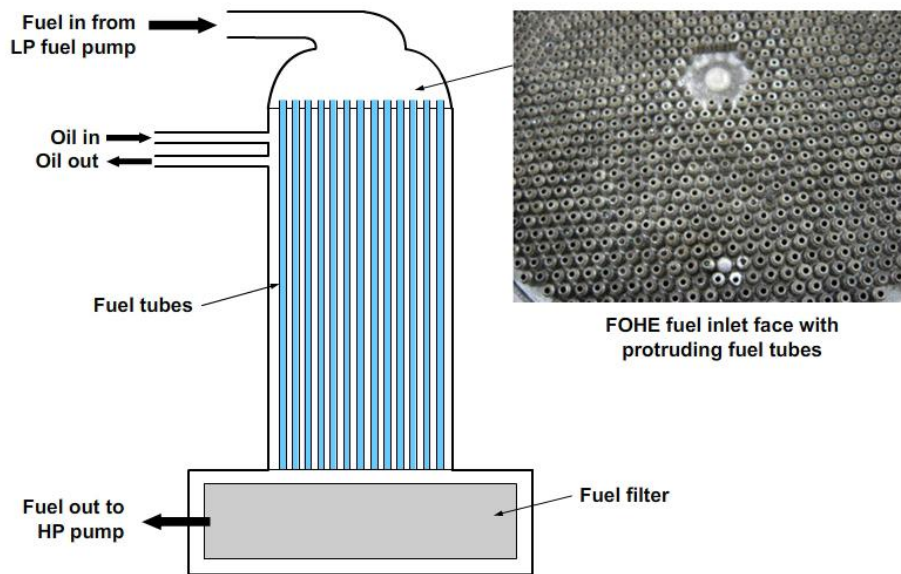
Fuel Oil Heat Exchanger (FOHE)
