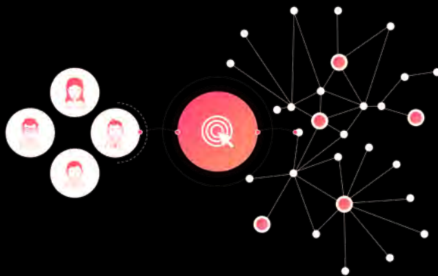
Lookalike
