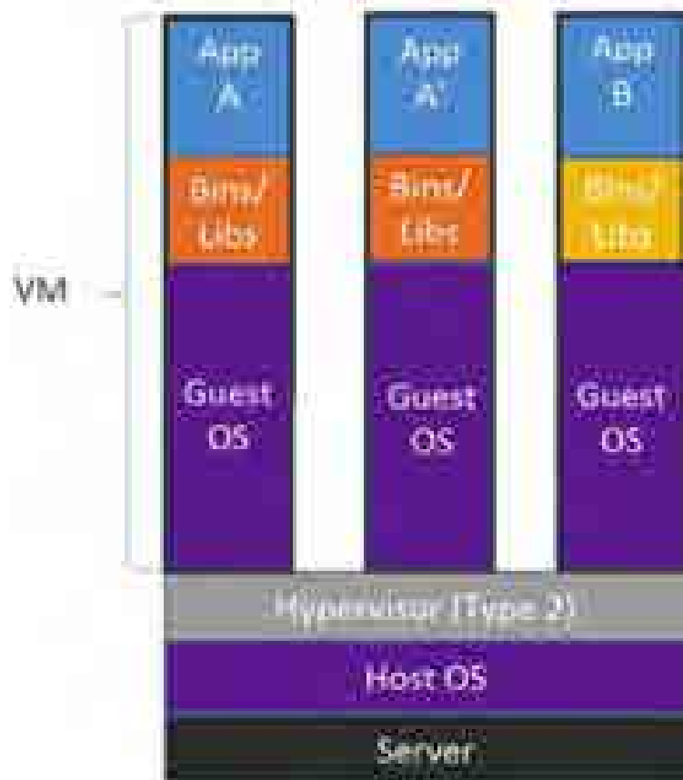
KVM/Xen/VMware
