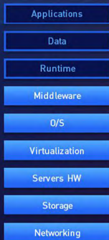
PaaS
